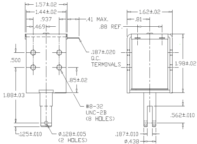
Solenoid shown energized with plunger fully seated
