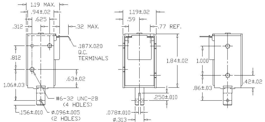
Solenoid shown with plunger fully seated in latched position
